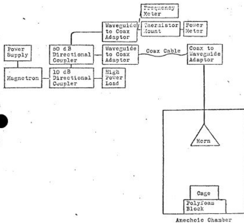
Fig. 1. Schematic diagram of the apparatus.
